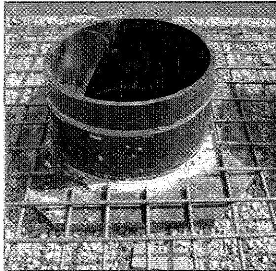
A reinforced concrete pad for H-20 traffic loading
