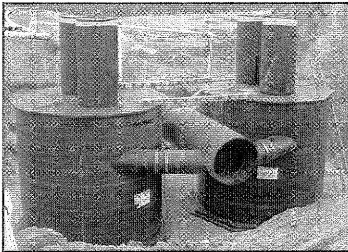
Custom designed AS-9 Twin, Aqua-Swirl™
