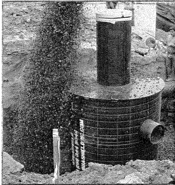
Class I backfill material around the Aqua-Swirl™
